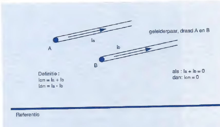
Figuur 2 Common mode (CM) en differential mode (DM) stromen
